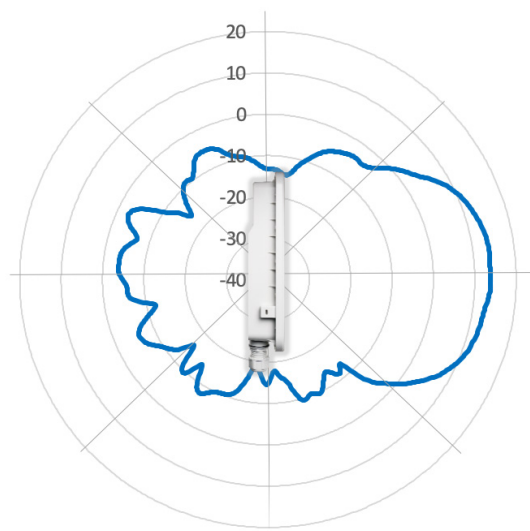
2.4 GHz Elevation
