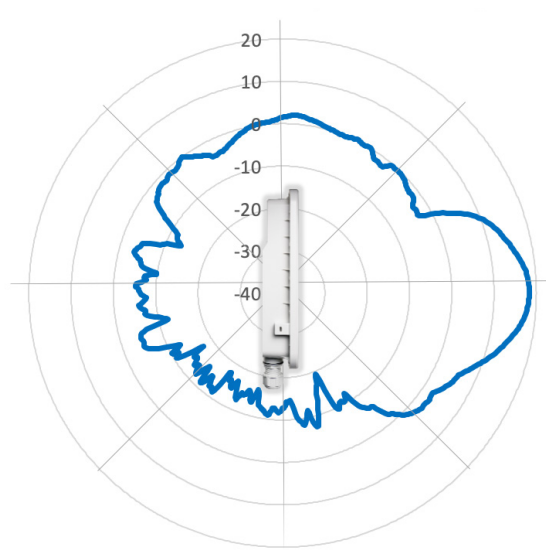
5 GHz Elevation
